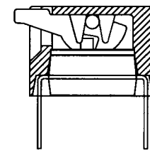
"H" Terminal
